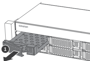
3.5-inch HDD
